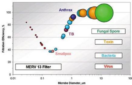
HVAC System with particulate filter only
